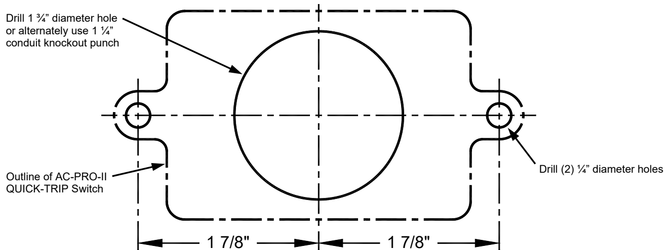
Figure H: AC-PRO-II QUICK-TRIP Switch Drilling Plan
